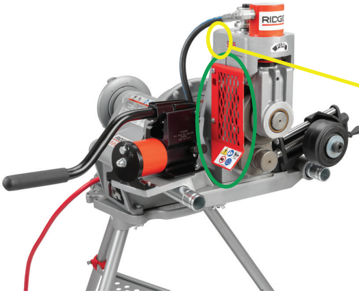
Figure 1 – RIDGID® 918 Roll Groover
